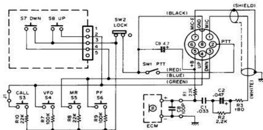
MC-44 SCHEMATIC DIAGRAM
